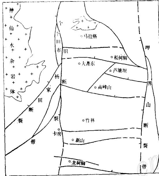
图2 个旧矿田地质构造略图 ⑤ Fig. 2. Sketch map of the Gejiu tin-polymetallic orefield, showing relationships of faults, granitic complexes and ore deposits.
