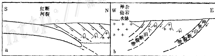
图3 a 南北向地质构造示意剖面图；b 东西向地质构造示意剖面图 Fig. 3. NS-trending geological sketch section across the Gejiu orefield (a) and EW-trending geological sketch section through the Gejiu orefield (b).
