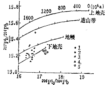
图 5 ^{207}\text{Pb}/^{204}\text{Pb} - ^{206}\text{Pb}/^{204}\text{Pb}
