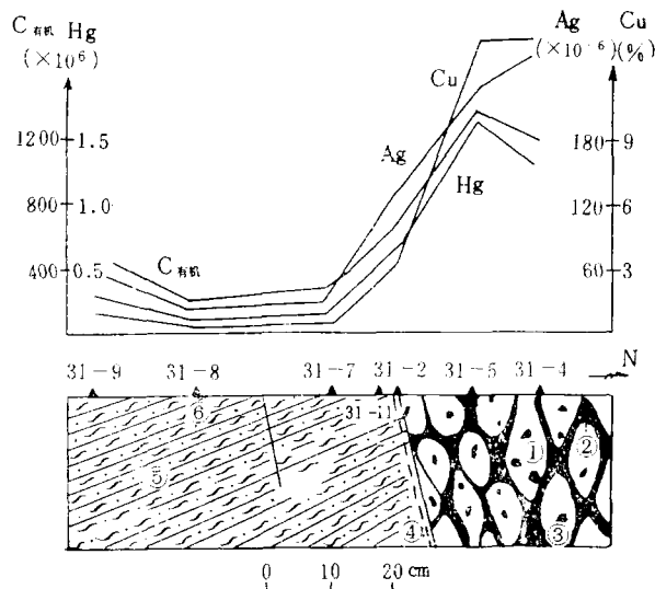
图2 东西向断裂的成矿作用(一坑1661中段主巷道) ①—构造透镜体；②—皮壳状富铜矿石；③—早期角砾状矿石；④—断裂面上的碳质物；⑤—浅色砂岩；⑥—采样位置 Fig. 2. Metallization of EW-trending fractures. 1—Tectonic lens; 2—Crustose Cu-rich ore; 3—Early brecciated ore; 4—Carbonaceous materials; 5—Light-colored sandstone; 6—Sampling location.
