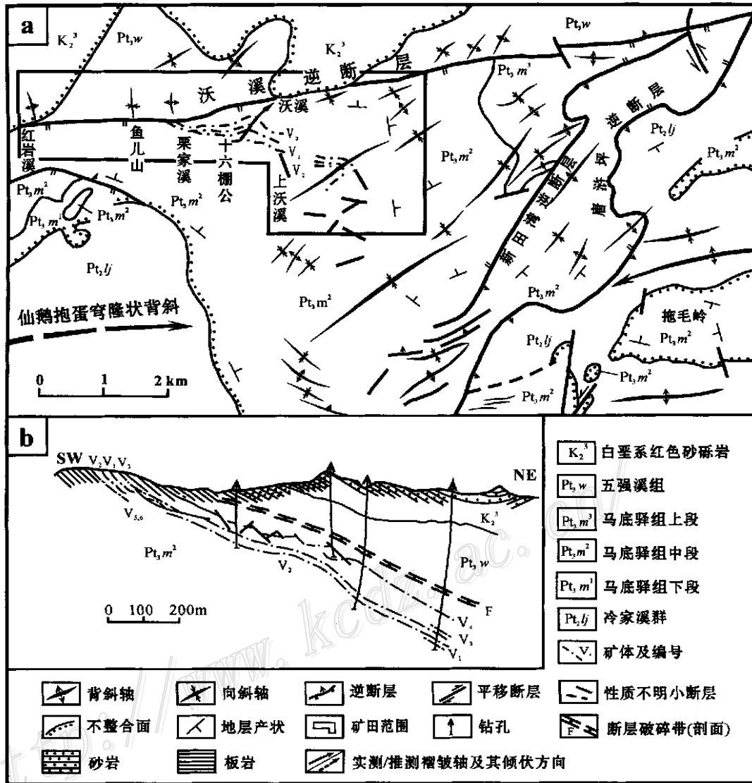
图1 沃溪矿田及邻区地质-构造略图(a)及沃溪矿床 NE-SW 向典型剖面图(b) (据罗献林等, 1996 修编) Fig. 1 Sketch map showing geological-structural features of the Woxi ore field and its adjacent areas (a) and typical NE-SW section of the Woxi deposit ( modified from Luo et al. , 1996)
