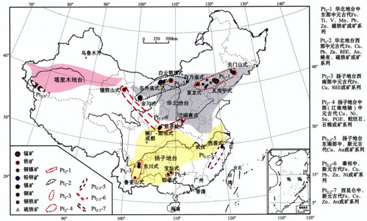
图 3 中元古代矿床成矿系列分布示意图 Fig. 3 Distribution map of the mineralogenic series during the Middle Proterozoic stage in China
