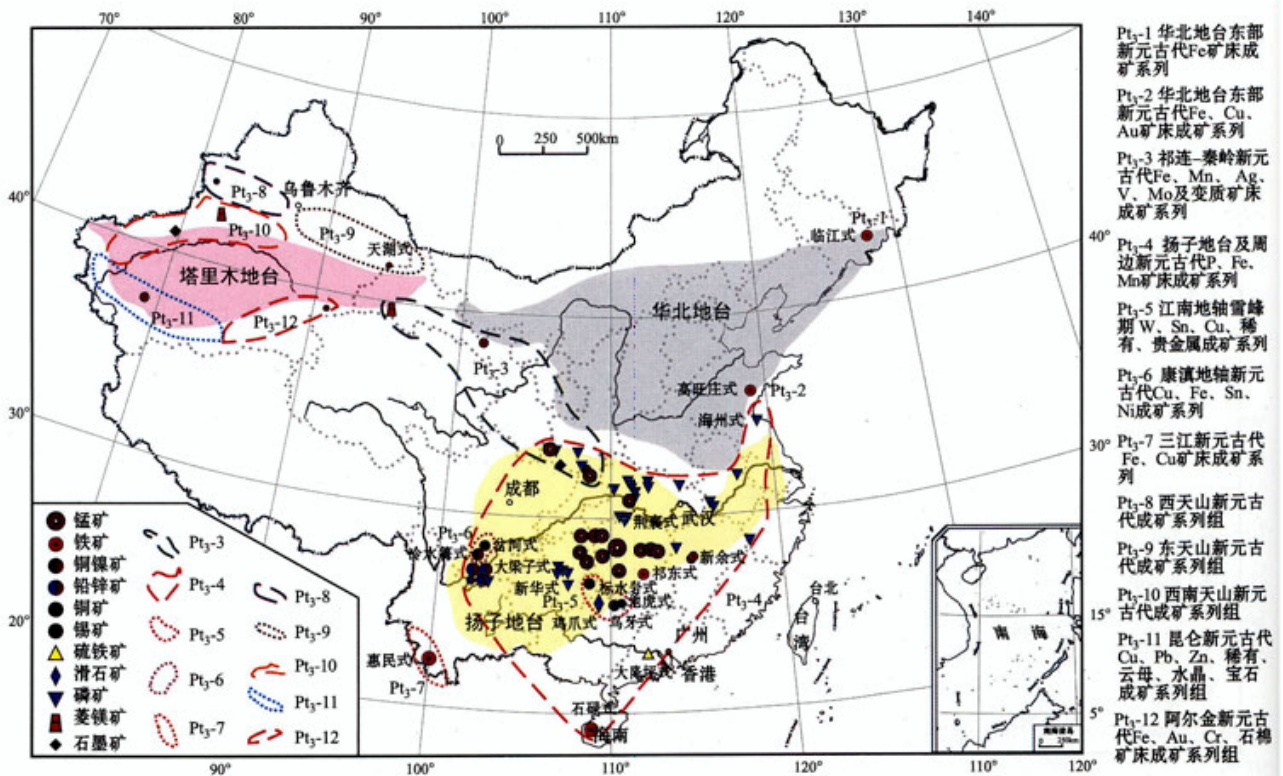
图 4 新元古代矿床成矿系列分布示意图 Fig. 4 Distribution map of the mineralogenic series during the Neoproterozoic stage in China
