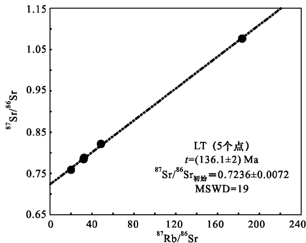
图4 烂头山钨锡矿床石英流体包裹体 Rb-Sr 等时线 Fig. 4 Rb-Sr isochron of quartz fluid inclusions in the Lantoushan W-Sn deposit
