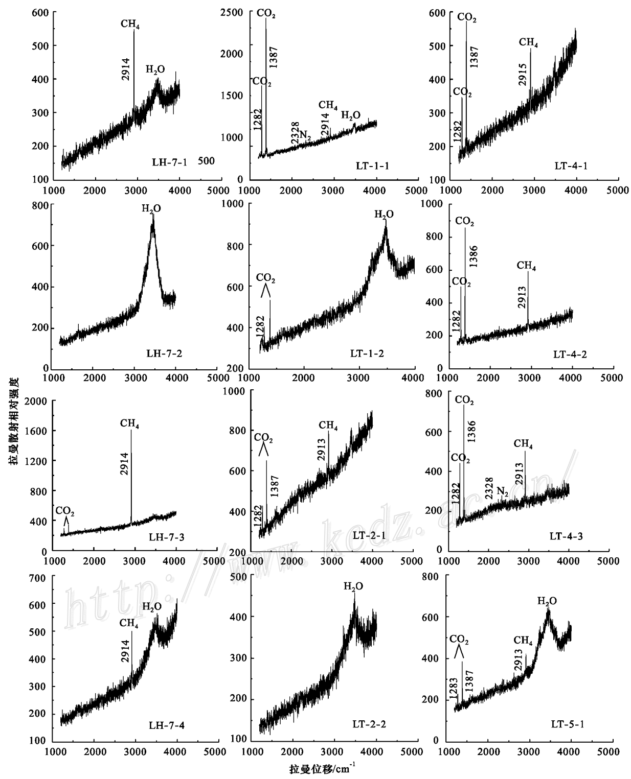
图 6 六合坳和烂头山矿床流体包裹体的激光拉曼光谱 Fig. 6 Laser Raman spectra of fluid inclusions from the Liuheao and Lantoushan deposits
