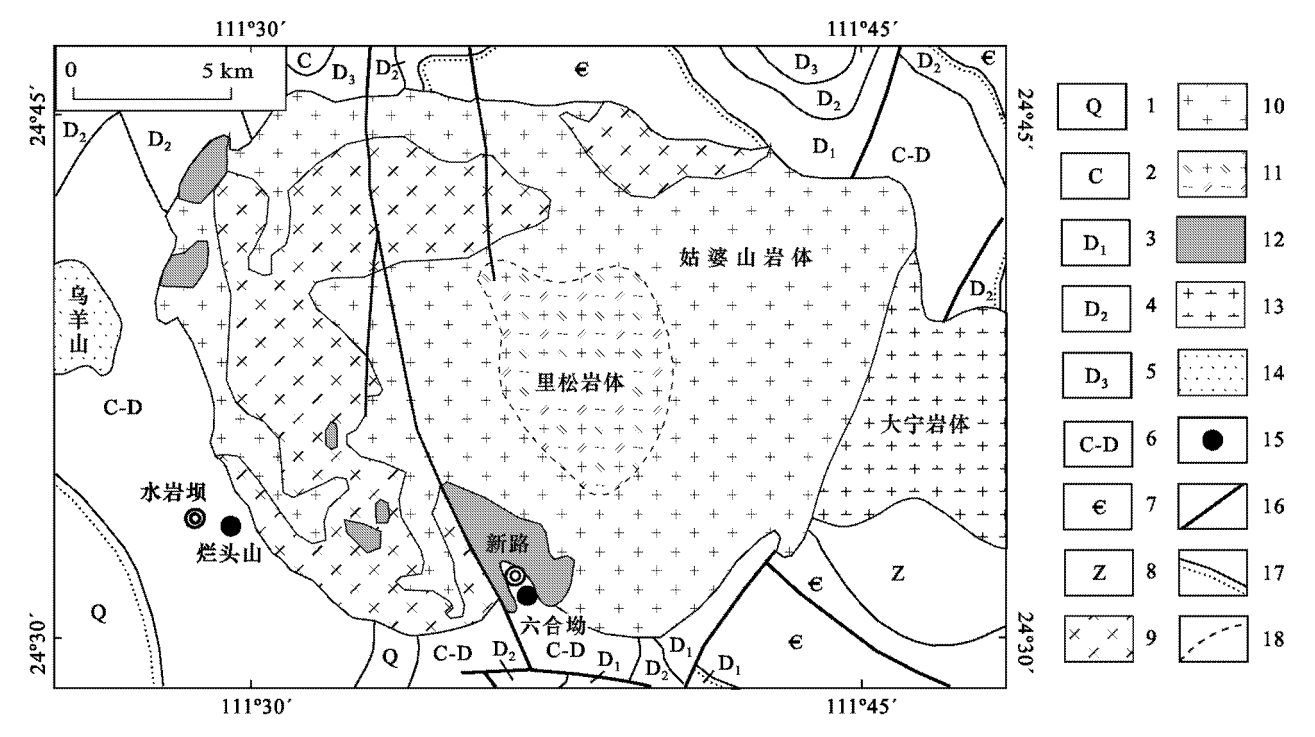
图 1 新路—水岩坝矿田地质略图(据张德全等,1985;冯佐海等,2002;顾晟彦等,2006a 资料改编) 1—第四系砂泥岩;2—石炭系灰岩;3—泥盆系下统灰岩;4—泥盆系中统灰岩;5—泥盆系上统灰岩;6—石炭系-泥盆系灰岩、砂页岩;7—寒武系砂页岩;8—震旦系变质砂岩;9—中细粒斑状黑云母花岗岩(姑婆山西体);10—中粗粒斑状黑云母钾长花岗岩(姑婆山东体);11—角闪黑云母二长花岗岩(里松岩体);12—细粒黑云母花岗岩(晚期小岩体);13—花岗闪长岩;14—花岗岩;15—矿床(点);16—断裂;17—不整合地质界线;18—推测地质界线 Fig. 1 Simplified regional geological map of the Xinlu-Shuiyanba ore district (modified from Zhang et al., 1985; Feng et al., 2002 and Gu et al., 2006a)
