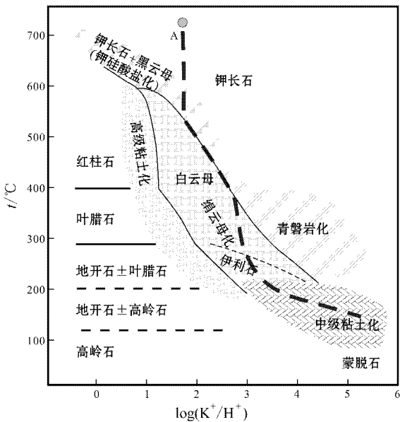
图9 斑岩铜矿床蚀变矿物稳定范围温度( K^+/H^+ )图解 (据 Hemley et al., 1964; Hedenquist et al., 1998a; Seedorff et al., 2005 修改)
