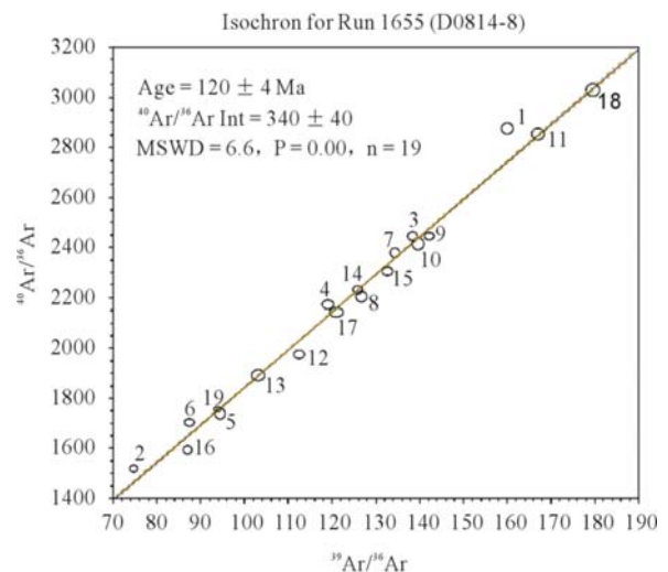
图2 样品D0814-8激光探 ^{40}\text{Ar}/^{39}\text{Ar} 等时线图
