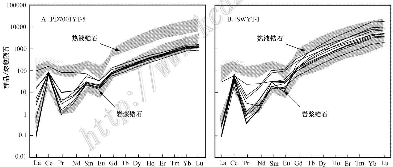
图6 锆石稀土元素球粒陨石标准化配分曲线(球粒陨石标准值引自 Sun et al., 1989, 底图据赵振华, 2010 修改) Fig. 6 Chondrite-normalized REE patterns of zircons (chondrite values after Sun et al., 1989, base diagrams modified after Zhao, 2010)
