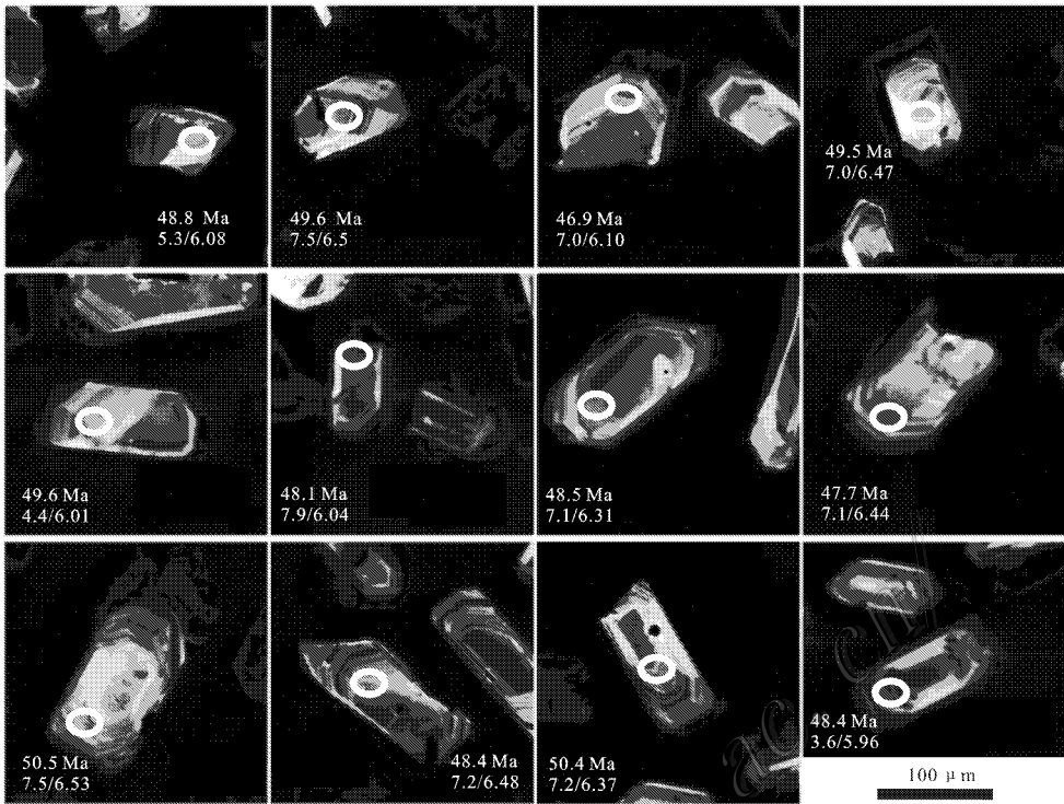
图 4 厅宫矿区斑状二长花岗岩 U-Pb、Hf 及 O 同位素原位分析锆石阴极发光 (CL) 图像及测试位置 Fig. 4 Cathodoluminescence (CL) images of representative zircons from the Tinggong porphyritic granite (sample TG-B037)
