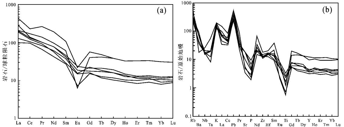
图 5 千家岩体花岗岩稀土元素球粒陨石标准化图解 (a) 和原始地幔标准化蛛网图 (b) (标准化数值依据 Sun et al., 1989) Fig. 5 REE patterns (a) and incompatible element spidergrams (b) of granitoids in Qianjia pluton (normalized data after Sun et al., 1989)
