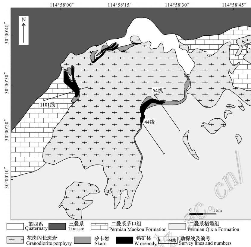
图3 龙角山矿床地质图(据纪云昊等,2019修改) Fig. 3 Geologic map of the Longjiaoshan deposit (modified after Ji et al., 2019)
